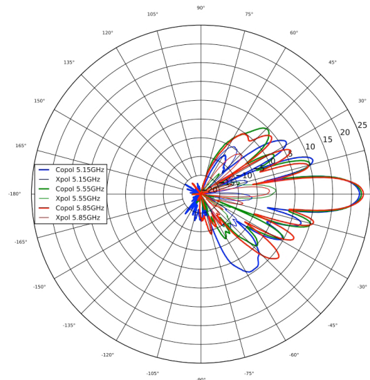
5 GHz Elevation
