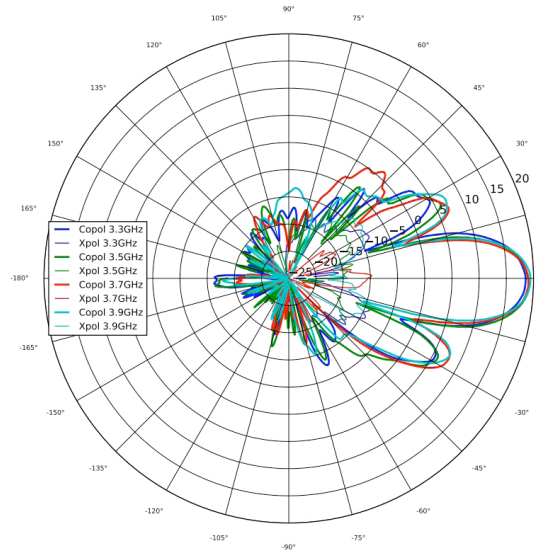
3 GHz Elevation
