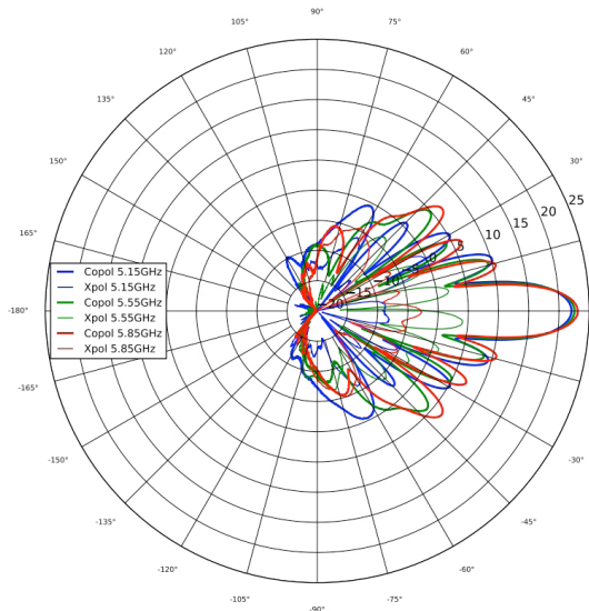
5 GHz Azimuth
