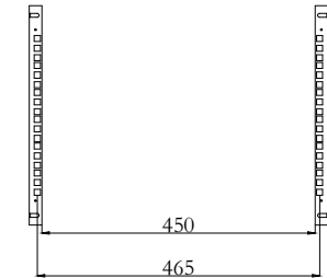
Mounting rails
