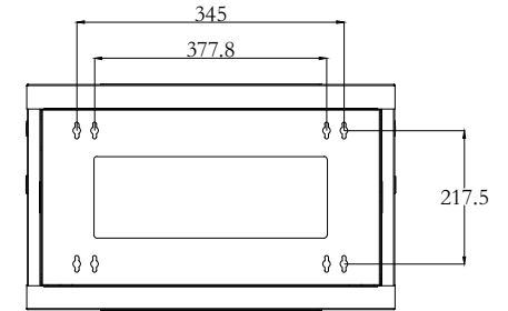
Back mounting holes
