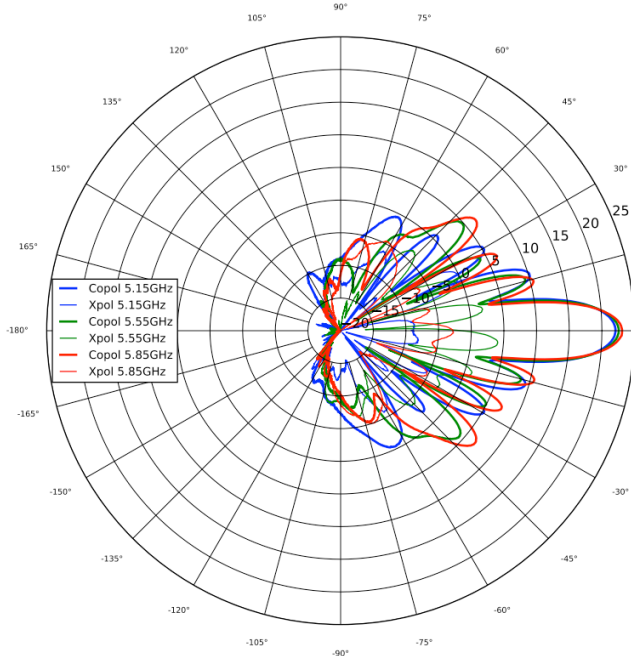
5 GHz Azimuth
