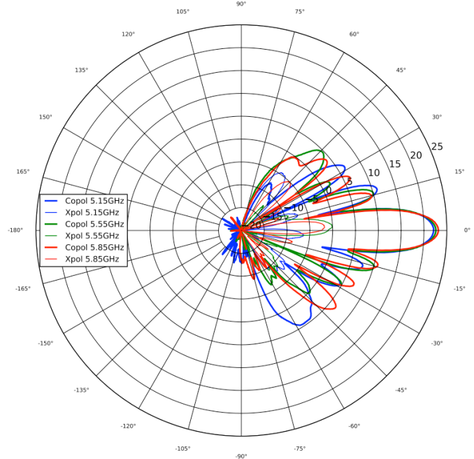
5 GHz Elevation
