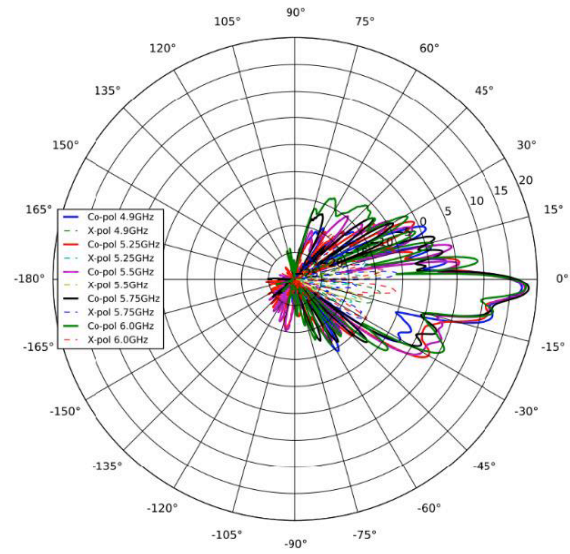
5 GHz Elevation
