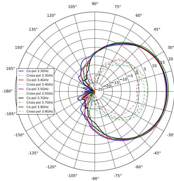
3 GHz Azimuth
