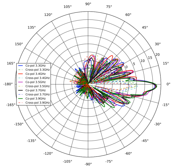
3 GHz Elevation
